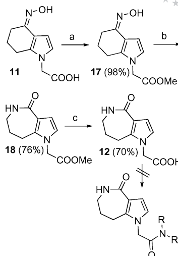
Scheme 5. Reagents and conditions: a) \text{SOCl}_2 , \text{MeOH} , reflux, 2 h; b) PPA, 120 °C, 15 min; c) \text{NaOH} , \text{MeOH}/\text{H}_2\text{O} .
