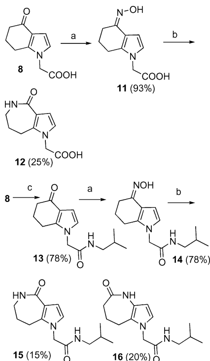
Scheme 4. Reagents and conditions: a) \text{NH}_2\text{OH}\cdot\text{HCl} , \text{AcONa} , \text{MeOH}/\text{H}_2\text{O} , room temp., 24 h; b) PPA, 120 °C, 15 min; c) \text{Me}_2\text{CHCH}_2\text{NH}_2 , DMTMM, NMM, THF, room temp., 12 h.
