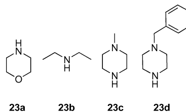
Figure 1. Structures of amines 23a–d .
