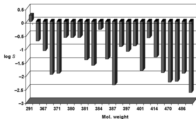
Figure 3. Distribution of molecular weight and log S in the array.
