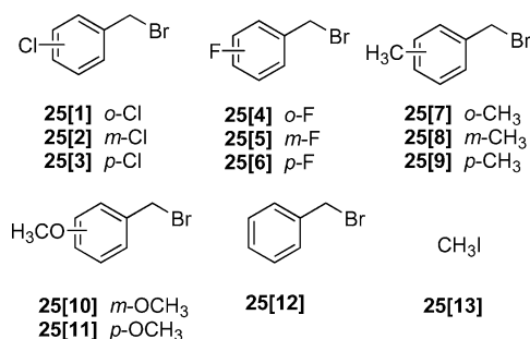
Figure 2. Structures of alkylating agents 25[1–13] .
