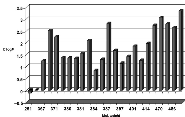
Figure 4. Distribution of molecular weight and log P in the array.
