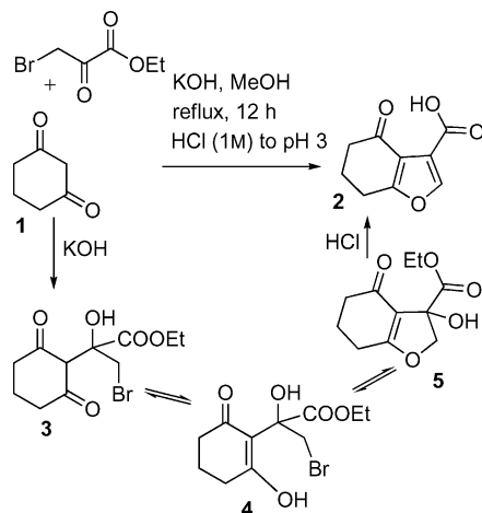
Scheme 2. Preparation of dihydrobenzofuran-3-carboxylic acid.
